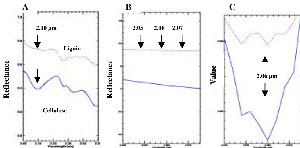
Figure 8. A: Spectral signatures of the plant biochemicals, lignin and cellulose, extracted from the USGS vegetation library B: A close up of these plant chemicals centered around 2.06 μm C: Continuum removed spectral signatures of the same chemicals shown in 8B.
