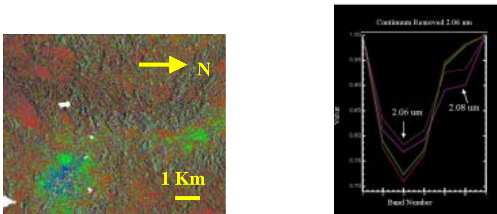
Figure 5. Subset of 2000 AVIRIS image shown on the left. A continuum removal has been applied to the 2.06 \mu\text{m} \text{CO}_2 absorption feature from 2.04 – 2.10 \mu\text{m} . The resulting image was density sliced into eight arbitrary color levels. The spectra on the right are average signatures extracted from selected density classes.
