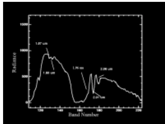
Figure 4. Spectral signature showing major CO 2 absorption regions
