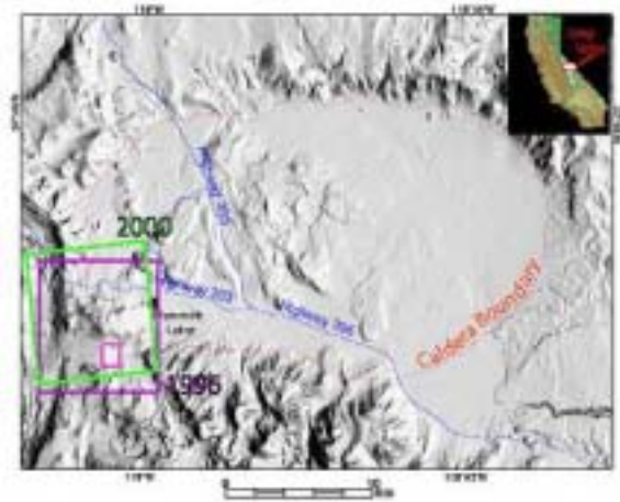
Figure 1. Shaded relief digital elevation model image of Long Valley Caldera. The scene boundaries of both years of AVIRIS data are shown as well as the approximate boundary of aerial photo and HyMap data scenes used.
