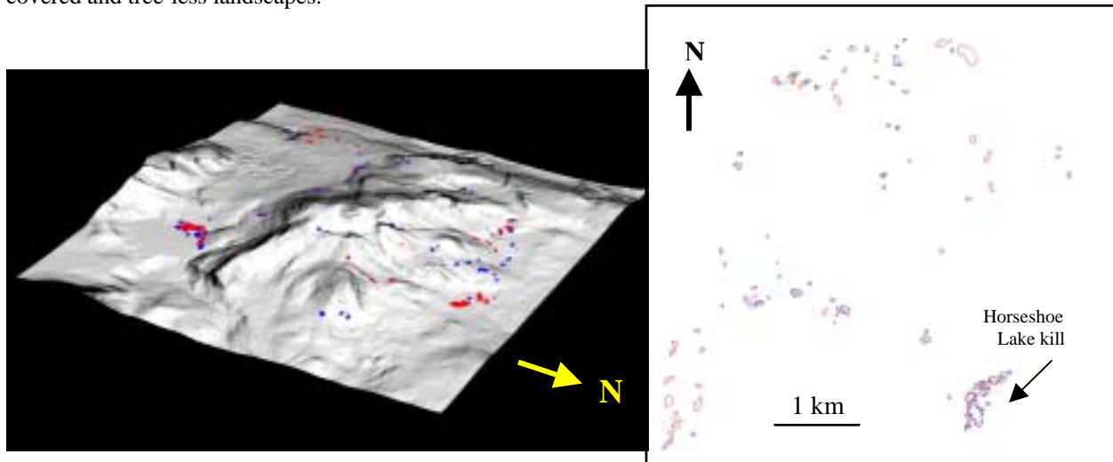
Figure 7. Left: results of MNF analysis of the 2.06 \mu\text{m} \text{CO}_2 absorption for 1996 (blue) and 2000 (red) AVIRIS imagery. Extreme MNF values from MNF band 2 (1996) and MNF band 3 (2000) shown draped on a shaded 10m USGS DEM. Right: Both years of extreme MNF values shown in plan view.
